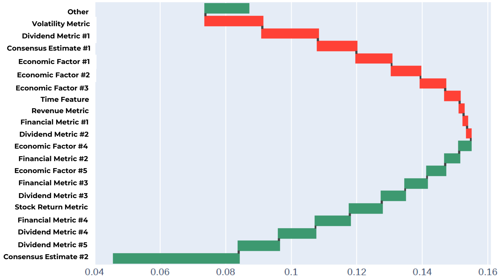
BG Model Prediction Breakdown Stock-Level Example: Dividend Growth Prediction of 8.7%
